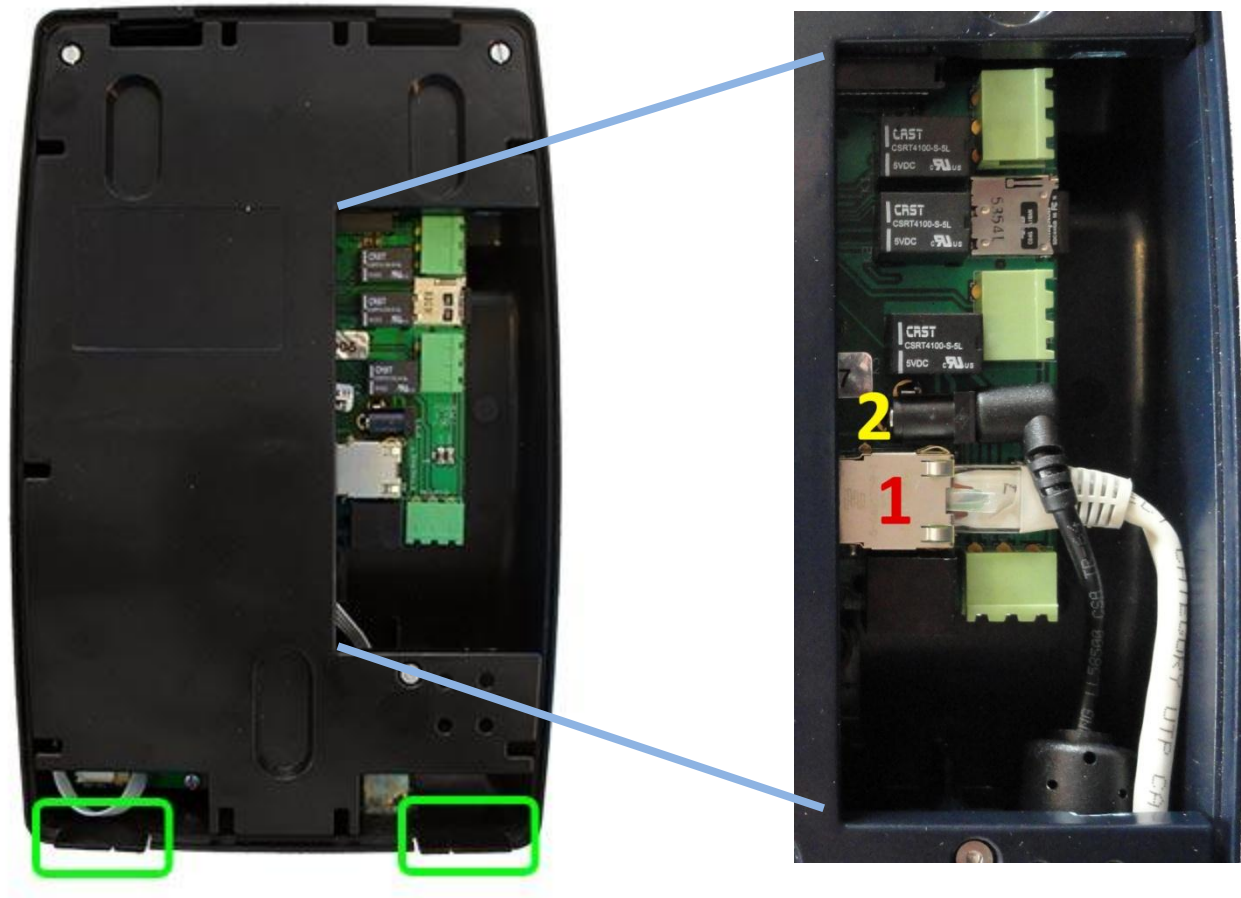
Back of the clock showing the breakouts in green and the network and power connectors
